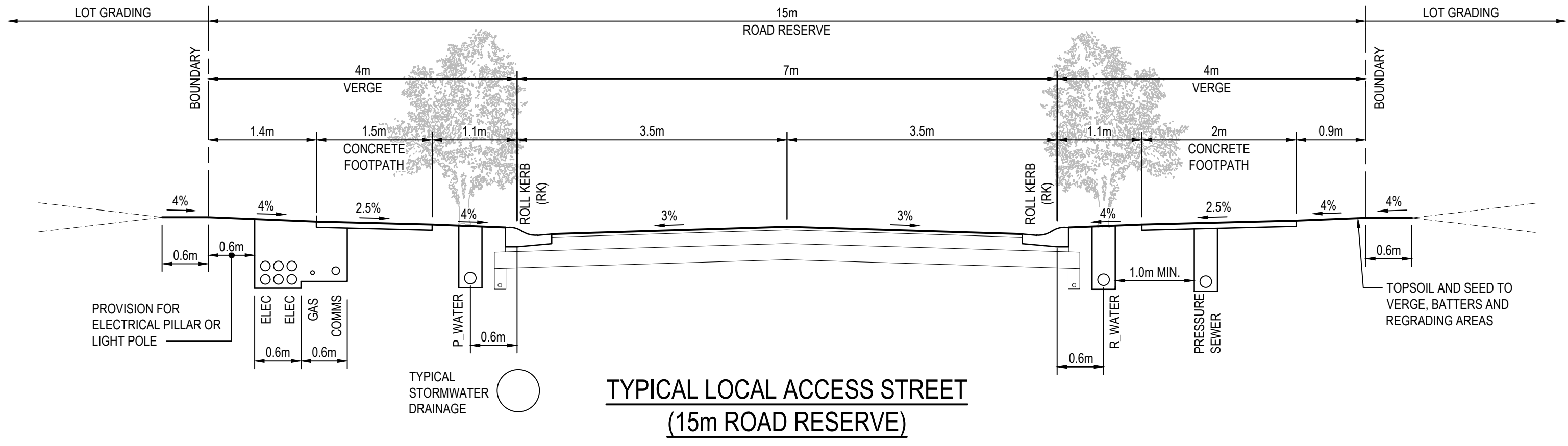
SECTION 5 SCALE 1:50 C1010 C1011
