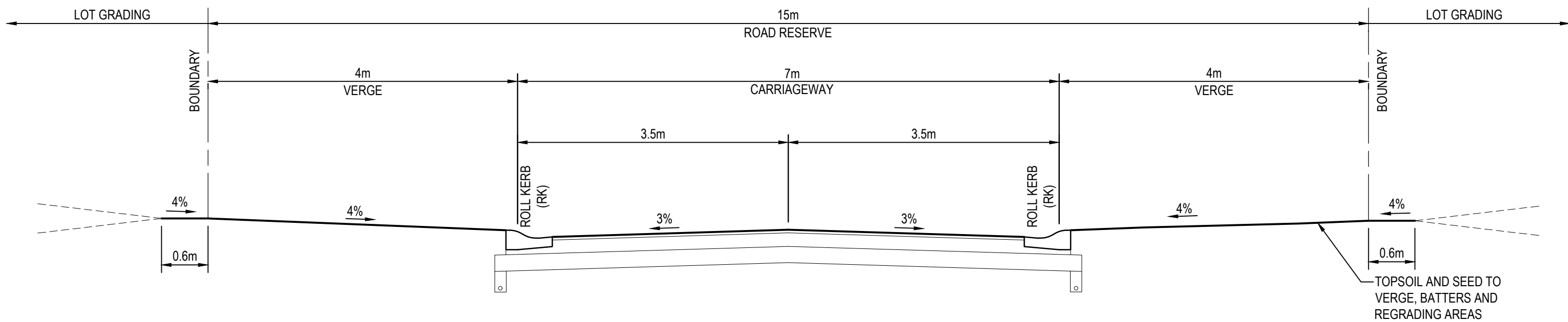
TYPICAL LOCAL ACCESS STREET (15m ROAD RESERVE)
