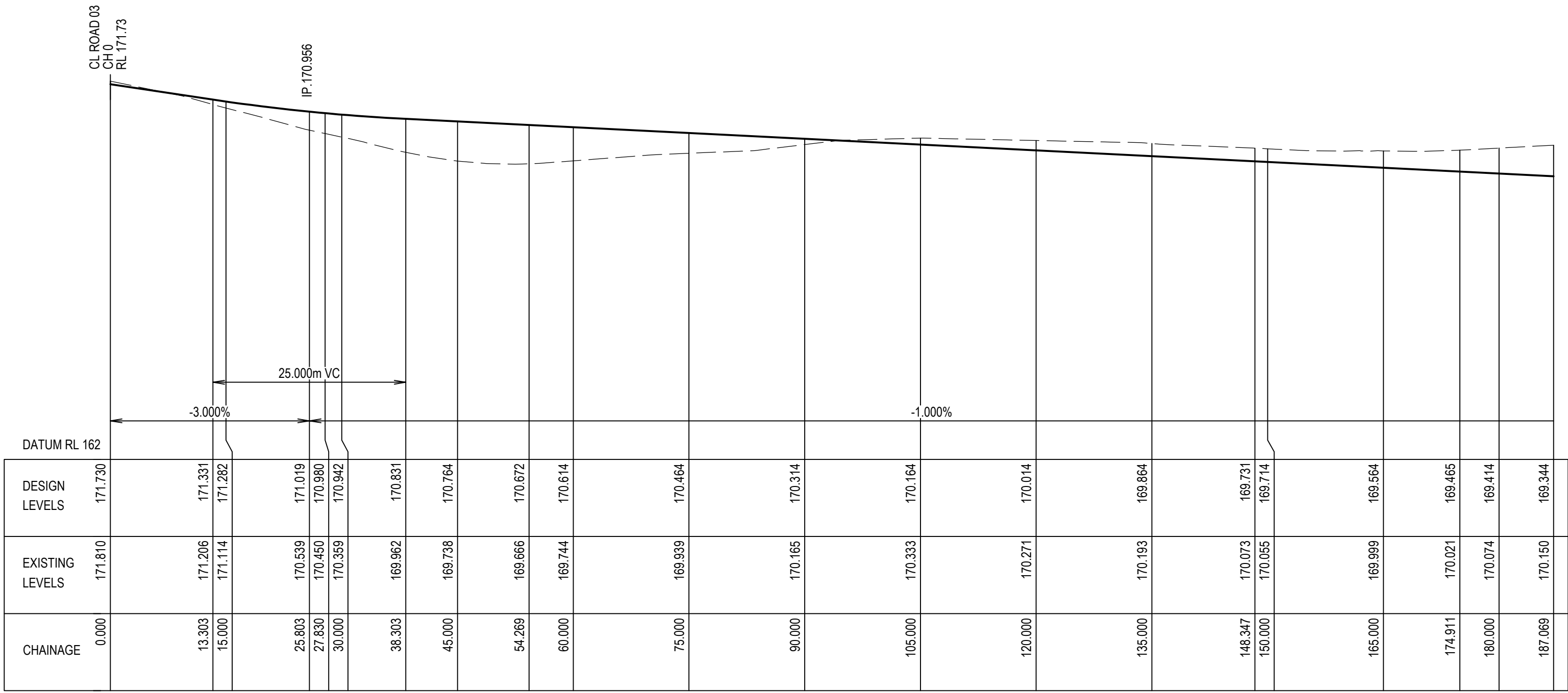
LONGITUDINAL SECTION - ROAD 09 SCALES: HORIZ 1:500 VERTICAL 1:100
