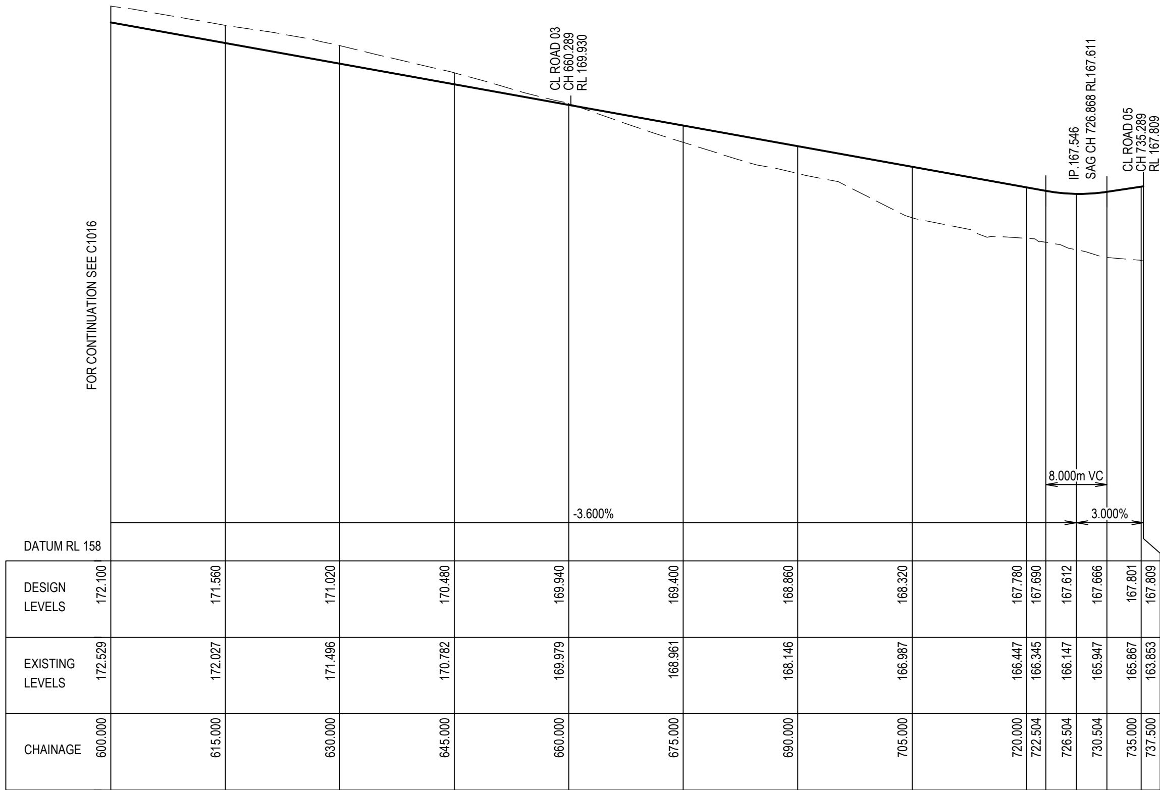
LONGITUDINAL SECTION - ROAD 01 SCALES: HORIZ 1:500 VERTICAL 1:100
