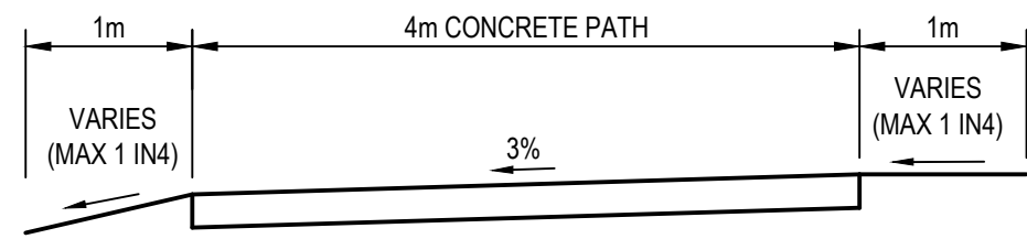
TYPICAL TYPICAL RIGHT OF WAY CROSS SECTION
