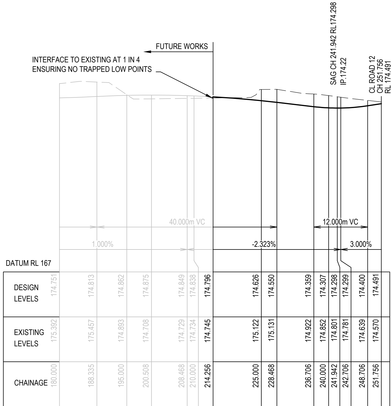
LONGITUDINAL SECTION - ROAD 15 SCALES: HORIZ 1:500 VERTICAL 1:100
