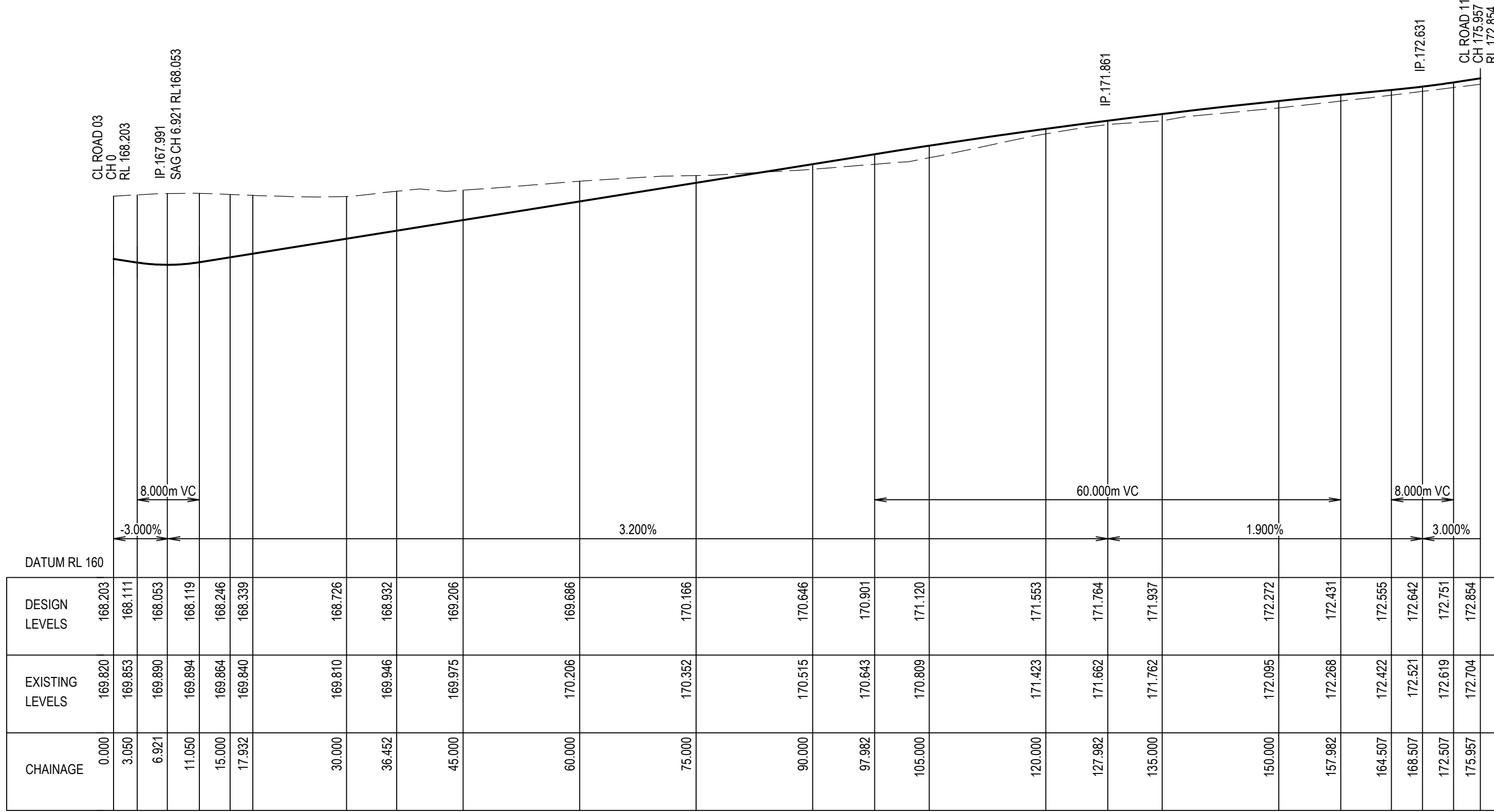
LONGITUDINAL SECTION - ROAD 08 SCALES: HORIZ 1:500 VERTICAL 1:100
