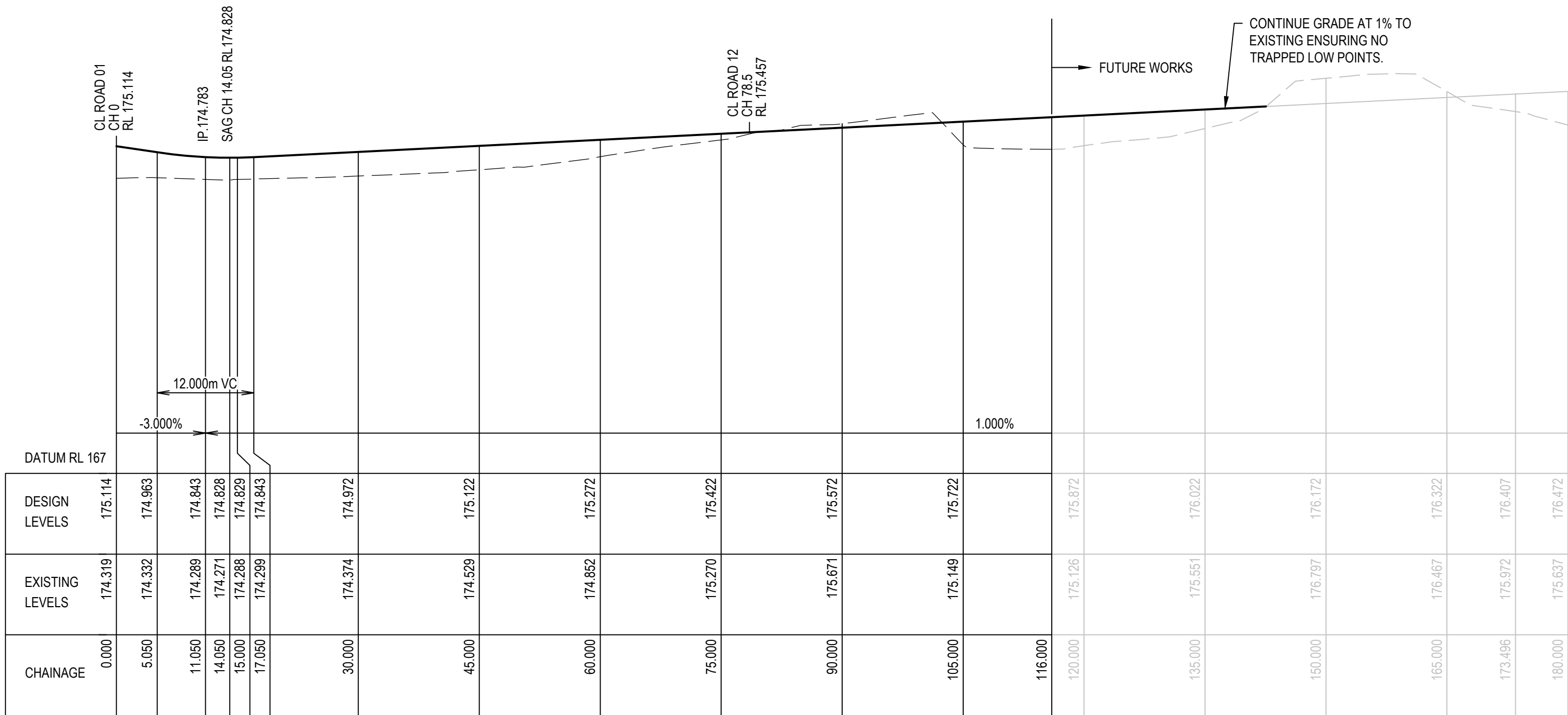
LONGITUDINAL SECTION - ROAD 04 SCALES: HORIZ 1:500 VERTICAL 1:100
