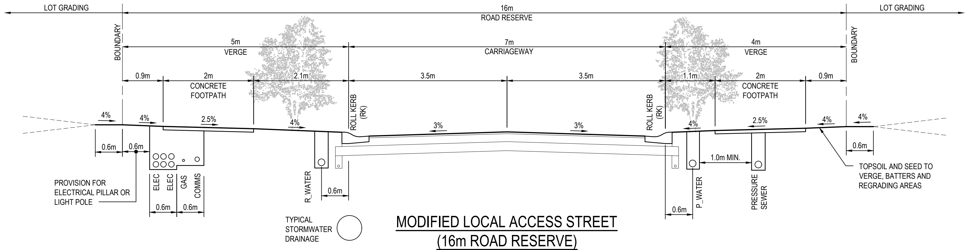
SECTION 4 SCALE 1:50 C1008 C1010
