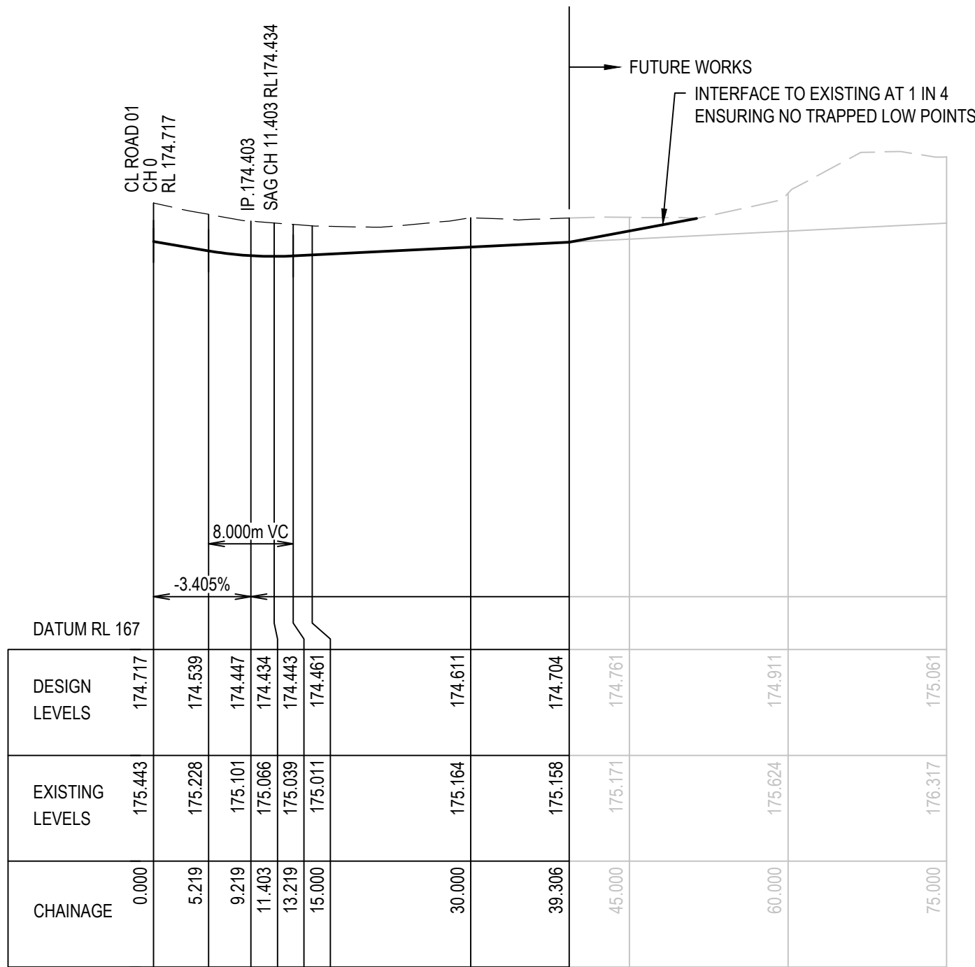
LONGITUDINAL SECTION - ROAD 02 SCALES: HORIZ 1:500 VERTICAL 1:100
