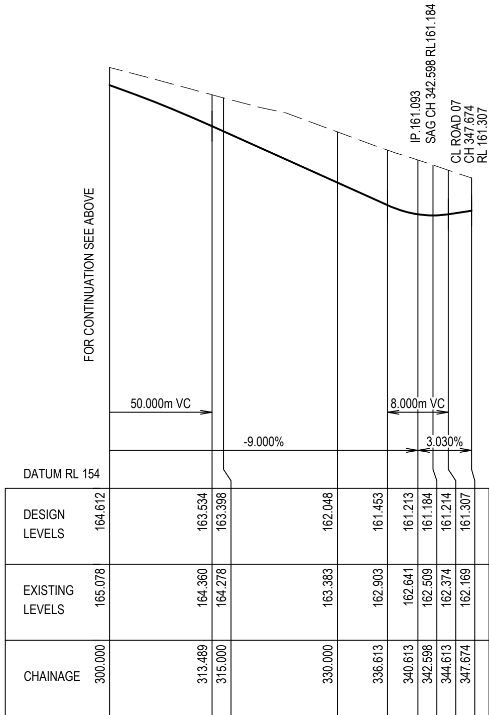
LONGITUDINAL SECTION - ROAD 05 SCALES: HORIZ 1:500 VERTICAL 1:100
