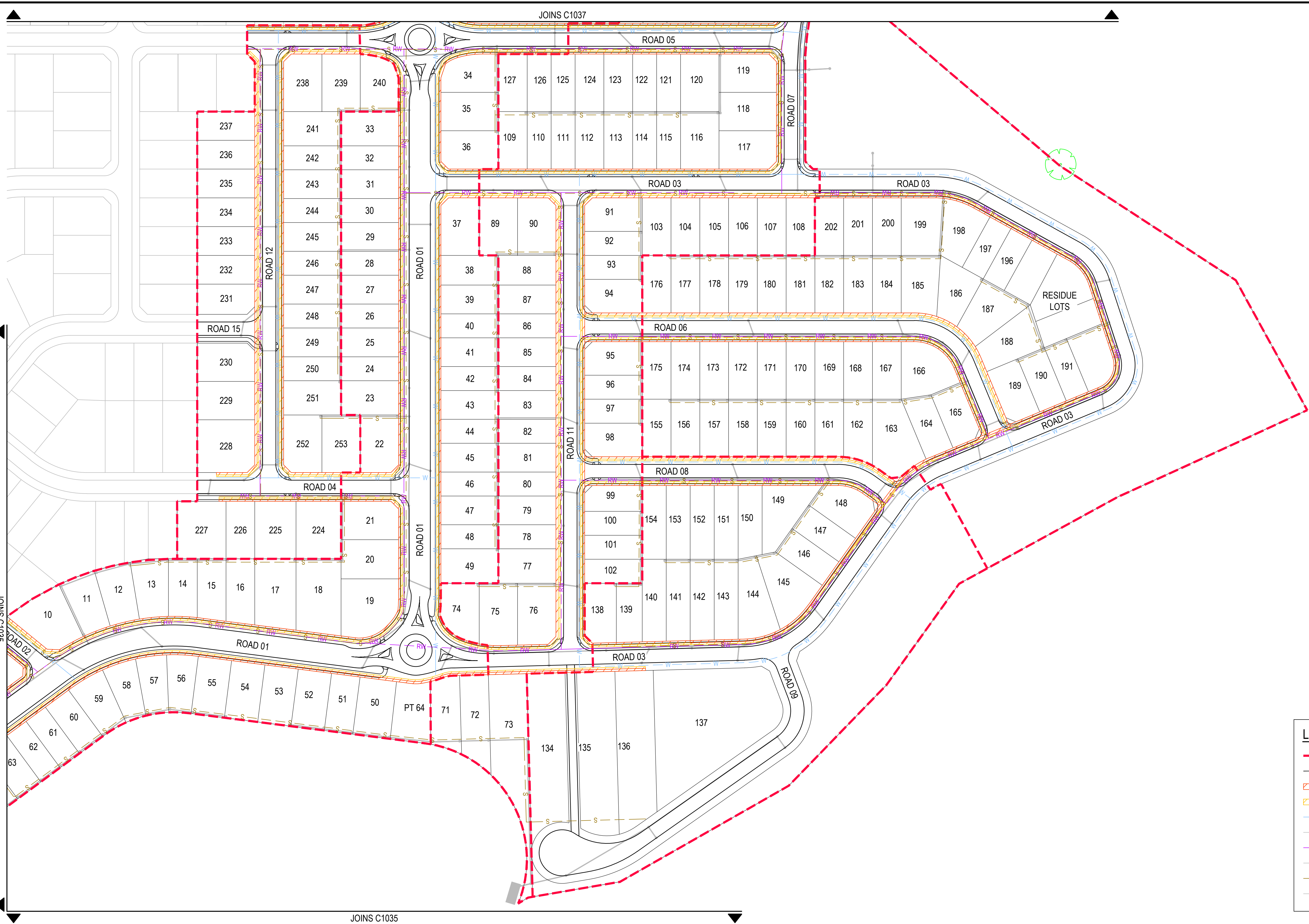
SERVICES LAYOUT SCALE 1:1000
