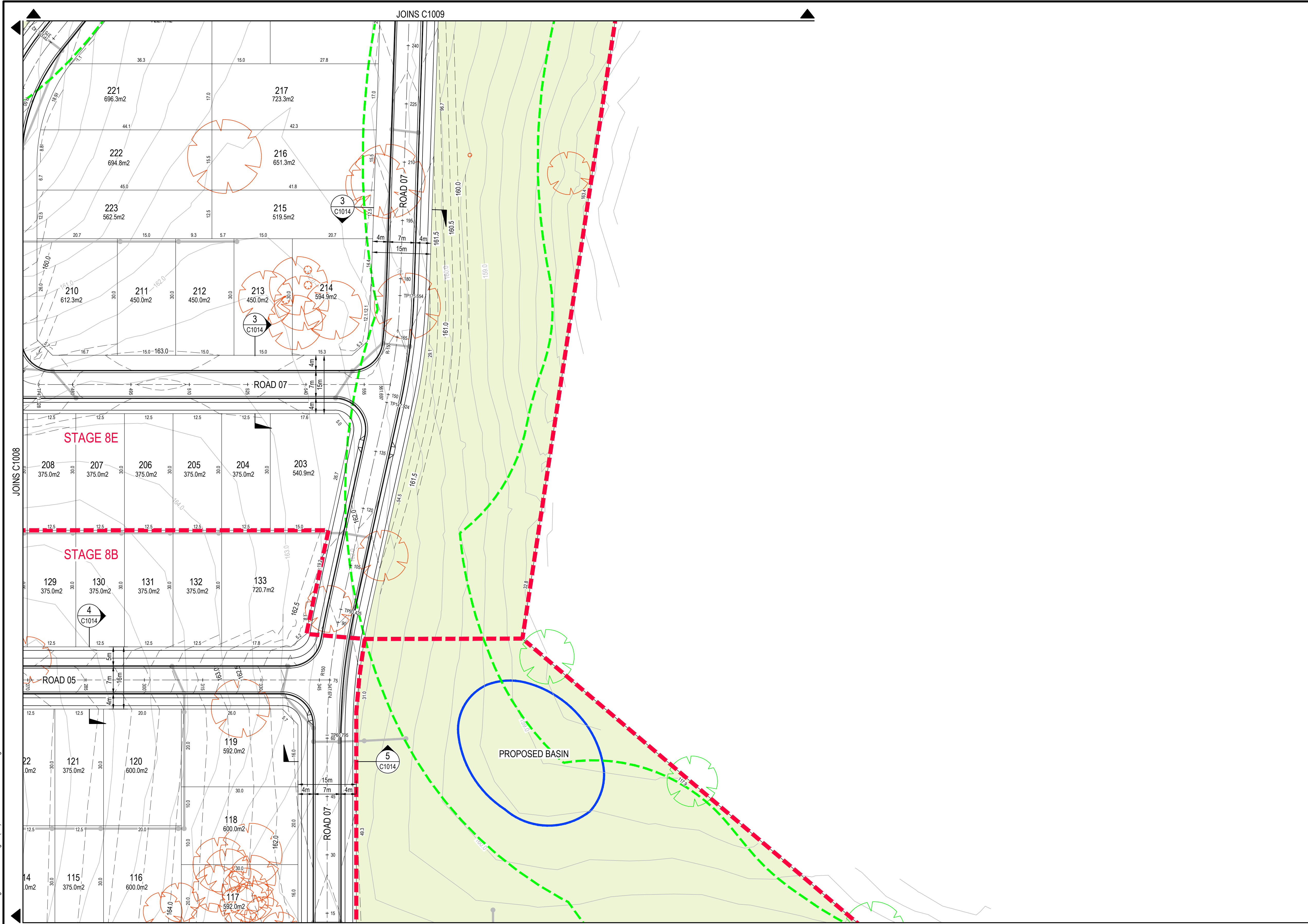
JOINS C1008 JOINS C1011 GENERAL ARRANGEMENT LAYOUT SCALE 1:500
