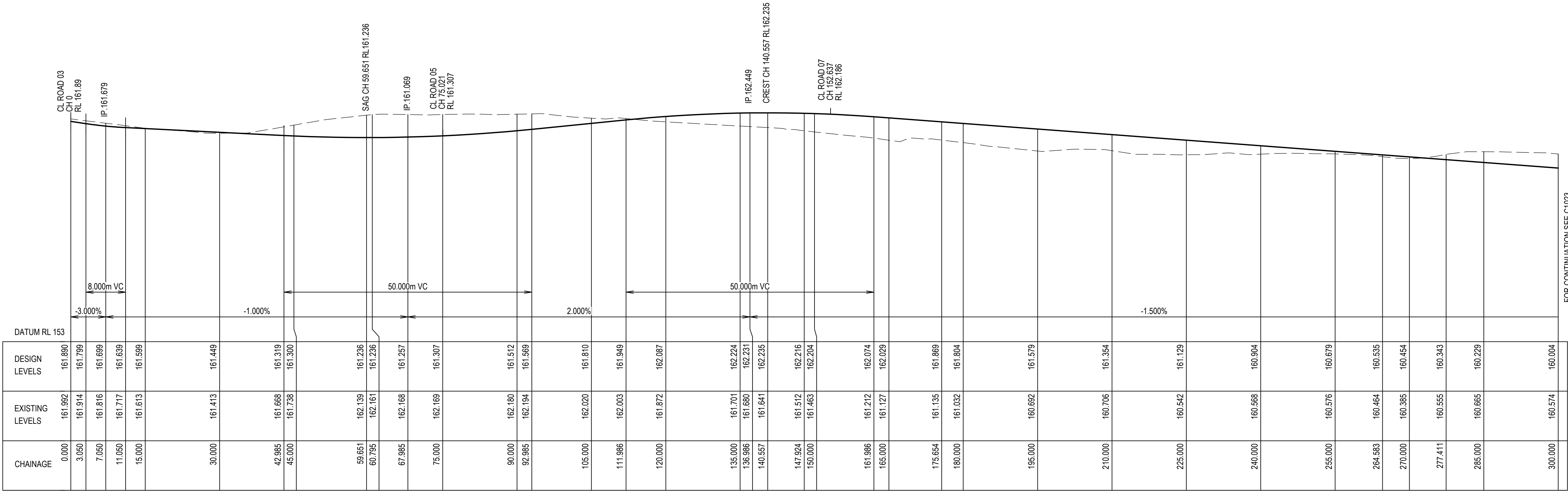
LONGITUDINAL SECTION - ROAD 07 SCALES: HORIZ 1:500 VERTICAL 1:100
