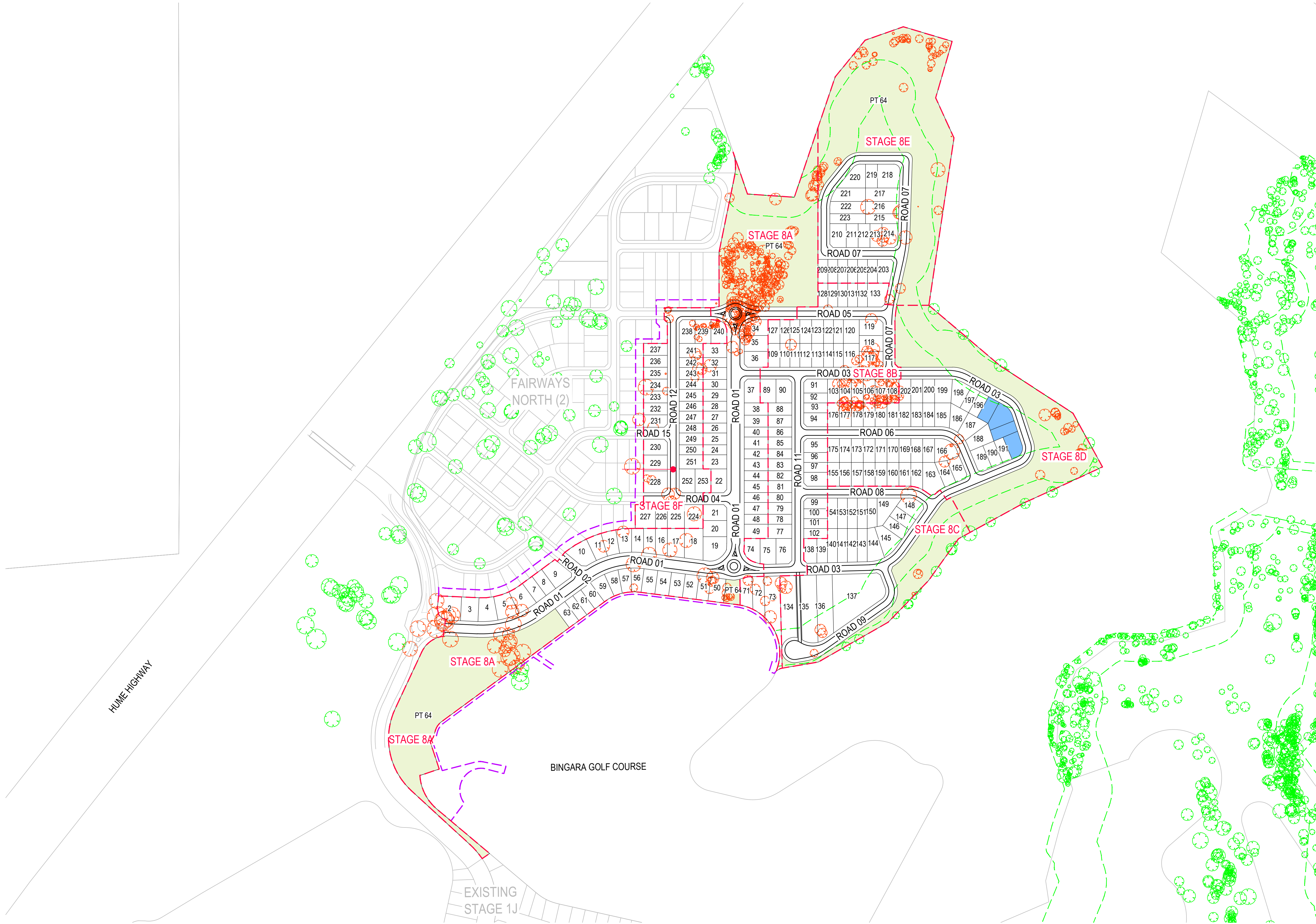
LOT LAYOUT SCALE 1:2500
