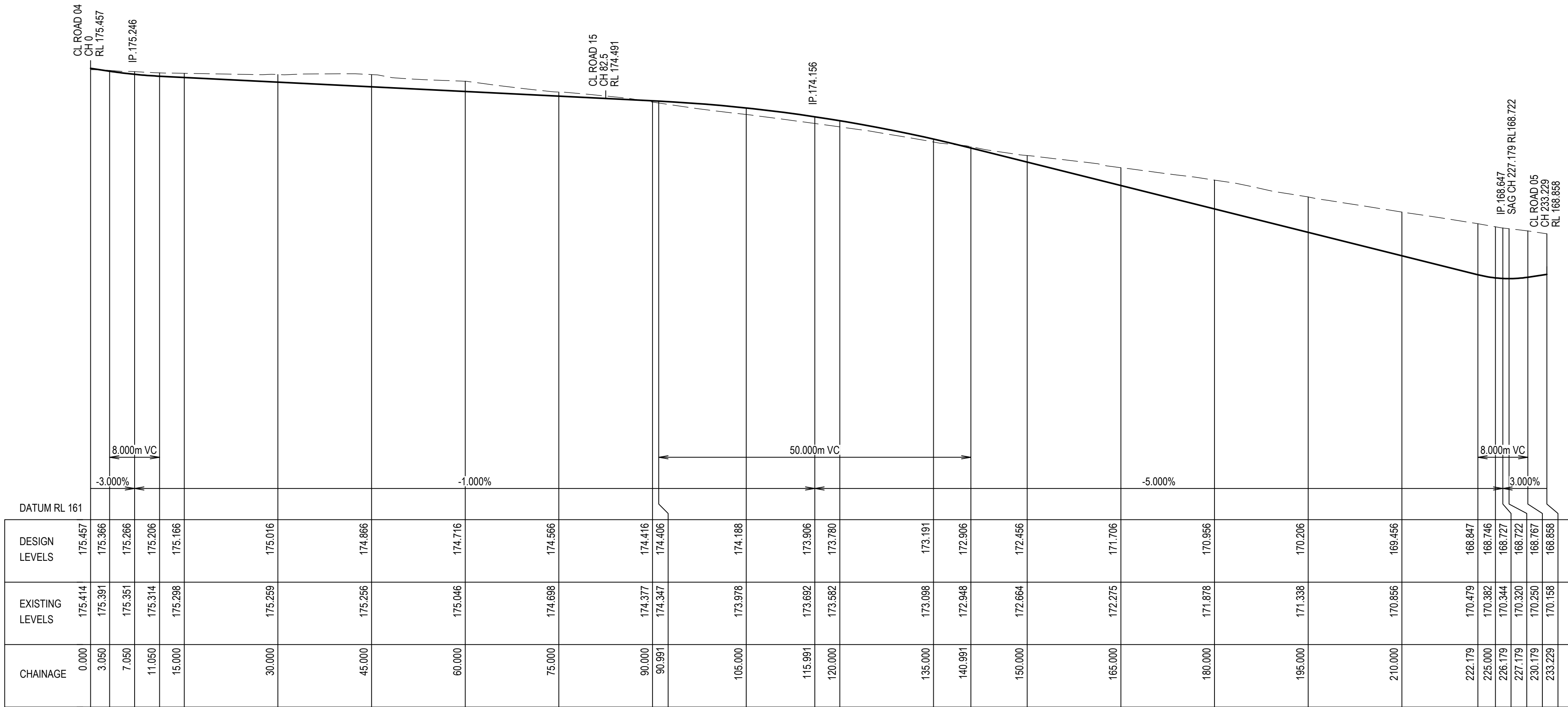
LONGITUDINAL SECTION - ROAD 12 SCALES: HORIZ 1:500 VERTICAL 1:100
