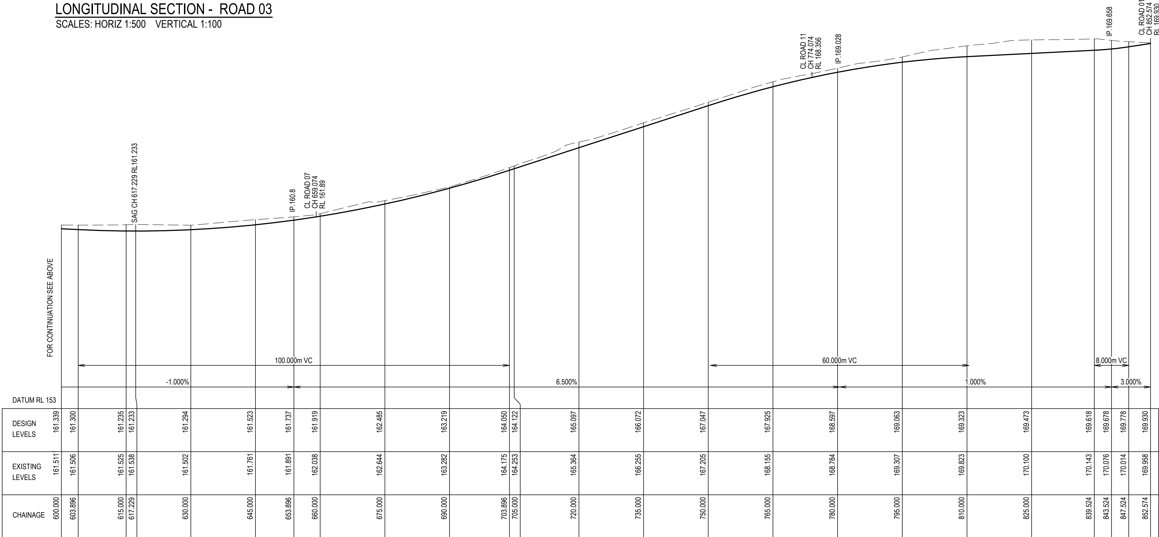
LONGITUDINAL SECTION - ROAD 03 SCALES: HORIZ 1:500 VERTICAL 1:100
