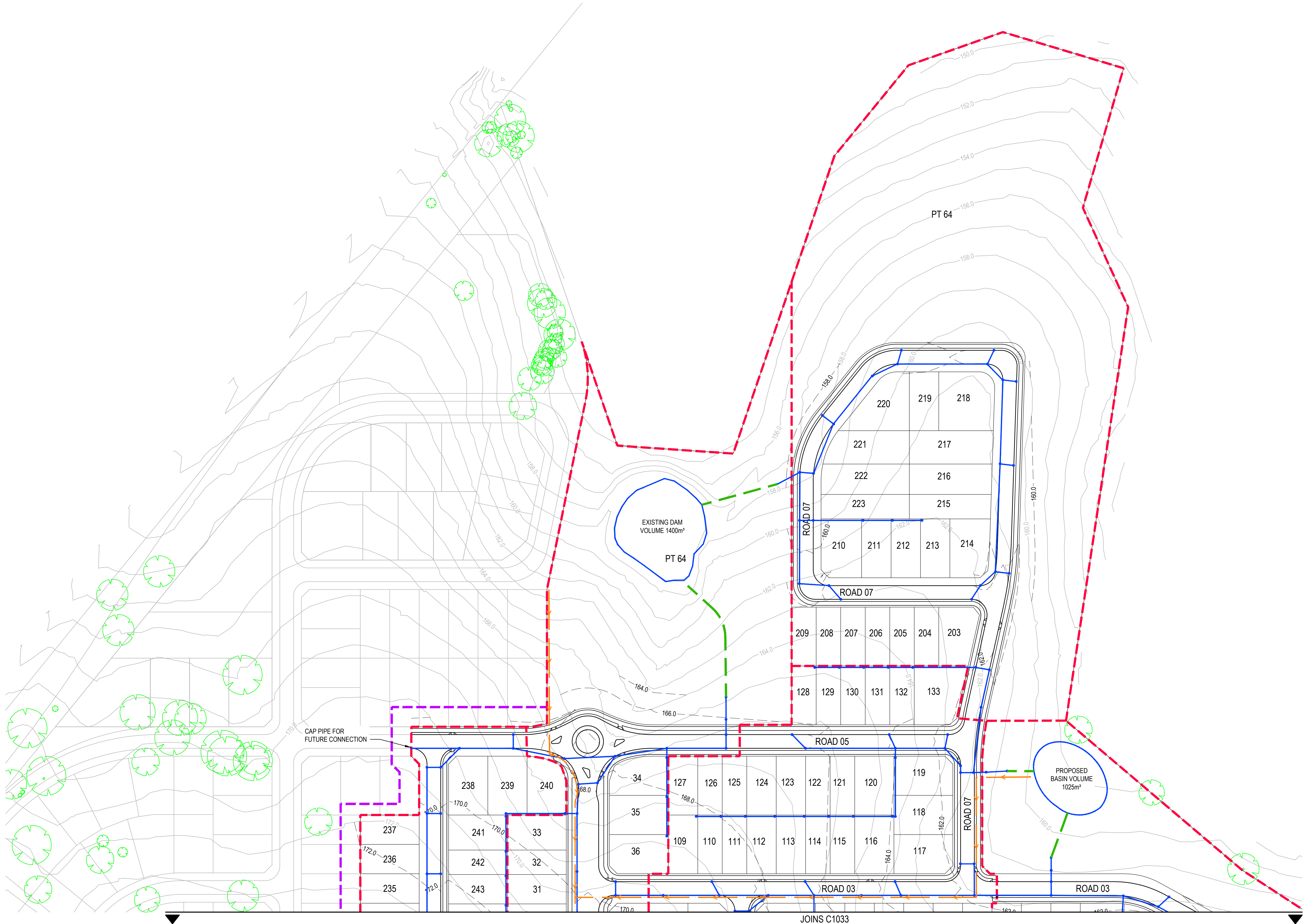
STORMWATER CONCEPT LAYOUT SCALE 1:1000
